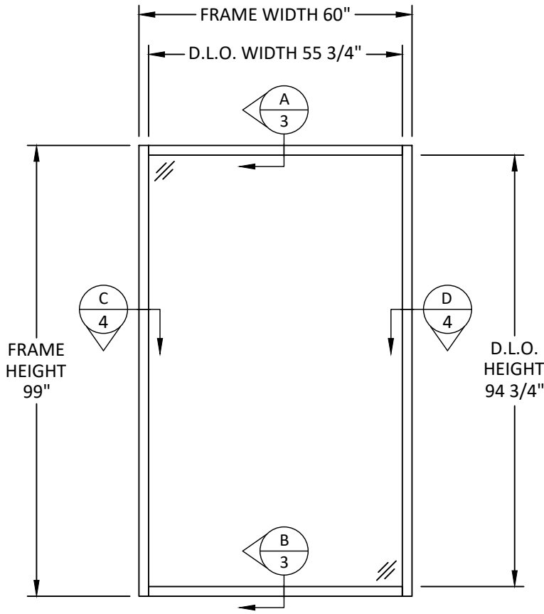
TYPICAL ELEVATION
