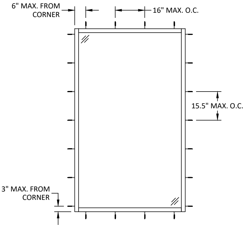
ANCHOR LAYOUT
